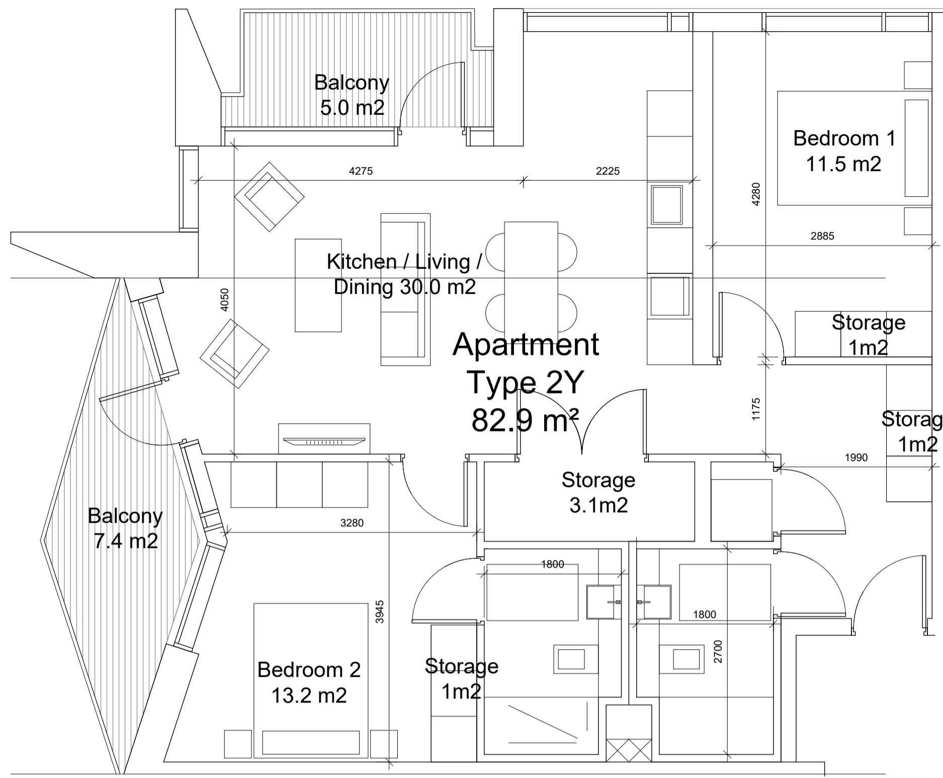
01 PL1928 2 Bed Apartment - Type 2Y (13 Unit) SCALE 1:50
