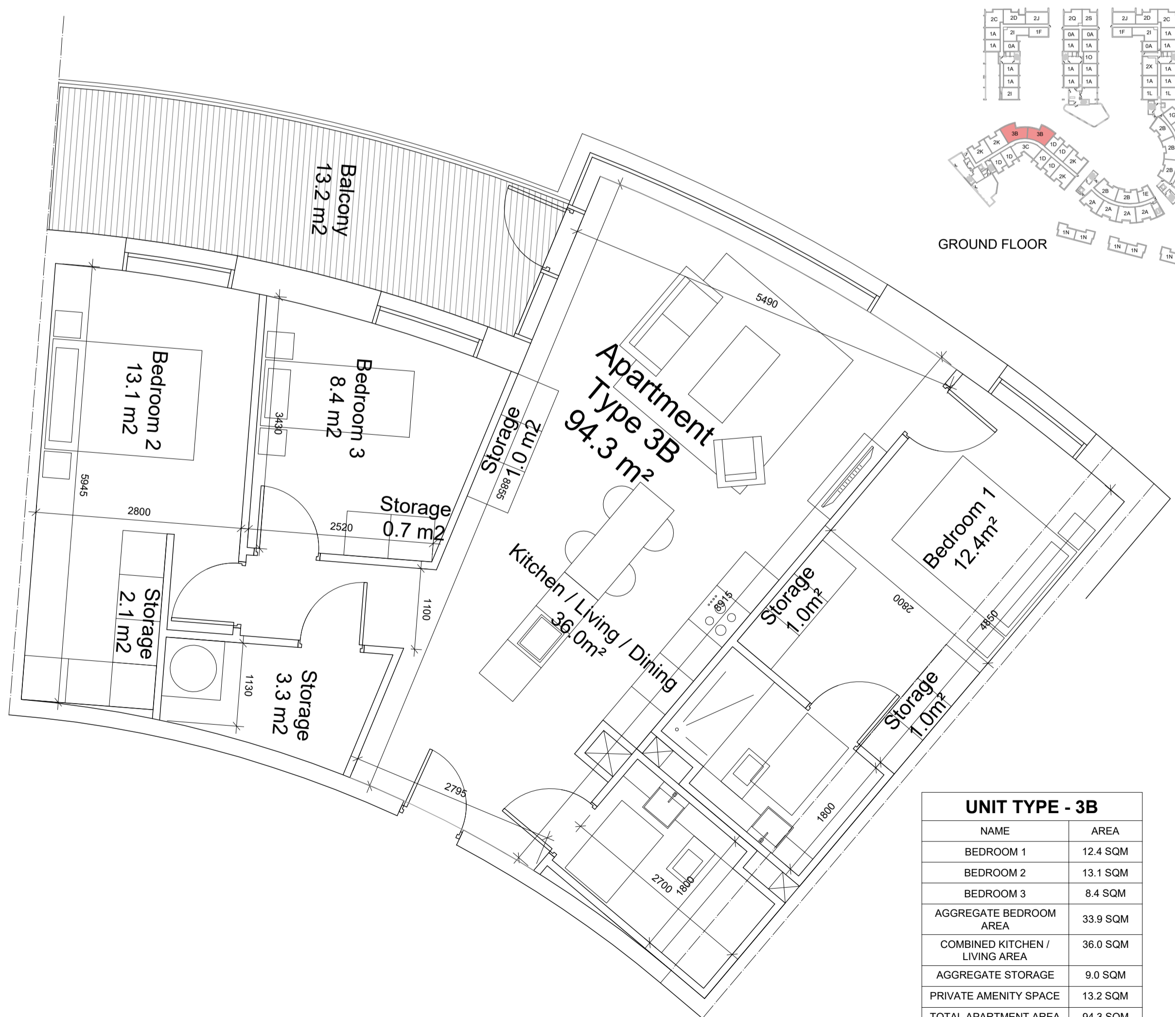
03 PL1928 3 Bed Apartment - Type 3B (8 Units) SCALE 1:50
