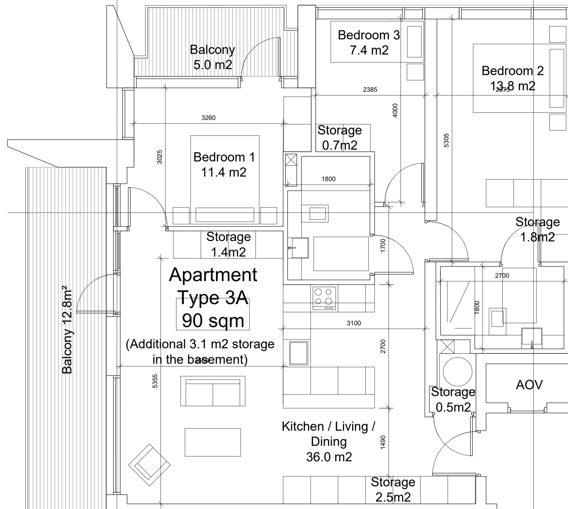
02 PL1928 3 Bed Apartment - Type 3A (1 Unit) SCALE 1:50
